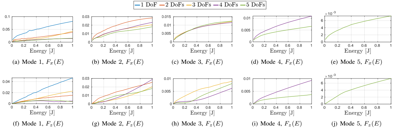
Fig. 6: Energy evolution of the modal integral Fréchet distance F(E) for the x (a)–(e) and z (f)–(j) backbone position.
