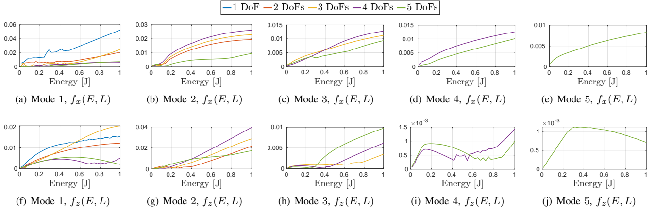
Fig. 5: Energy evolution of the modal Fréchet distance f(E, L) for the x (a)–(e) and z (f)–(j) tip position.
