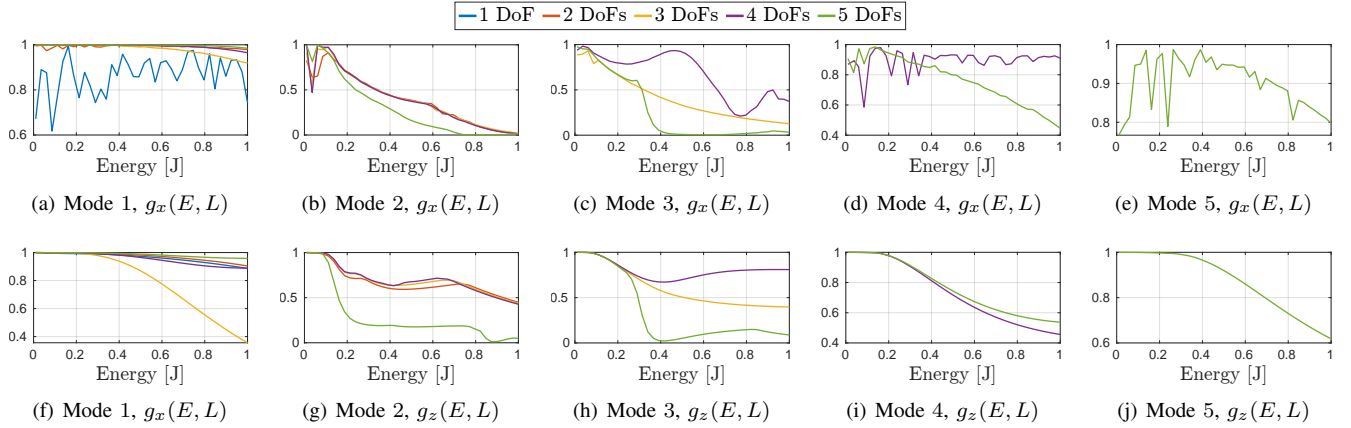
Fig. 7: Energy evolution of the modal coherence g(E, L) for the x (a)–(e) and z (f)–(j) tip position.
